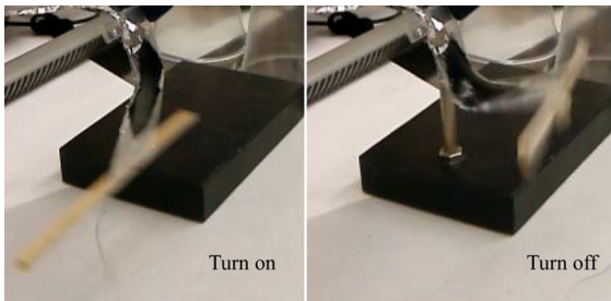
Fig. 16 Under the applied voltage of 5 kV and 3 Hz, gravity causes the joint to drive a larger inertia around the natural frequency, resulting in a joint angle of over 180°
