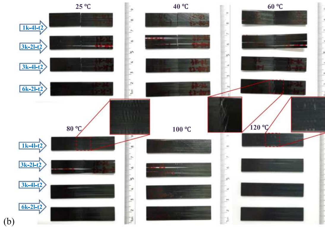
Fig. 10. Morphology of specimens undergone three-point bending, (a) laminates based on SMP-A and (b) laminates based on SMP-B.
