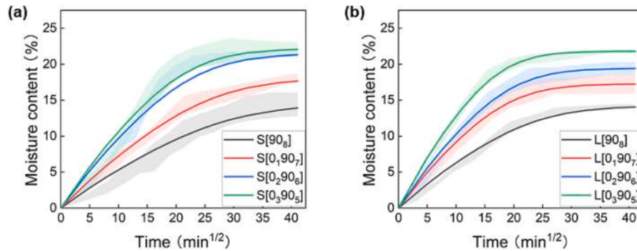
Fig 6. Experimental evolution of the water uptake for the square (S) and long rectangle (L) shaped hygromorphs with different stacking sequences and the predicting results (lines) by the 3D diffusion model. (a) square cases and (b) long rectangle cases.
