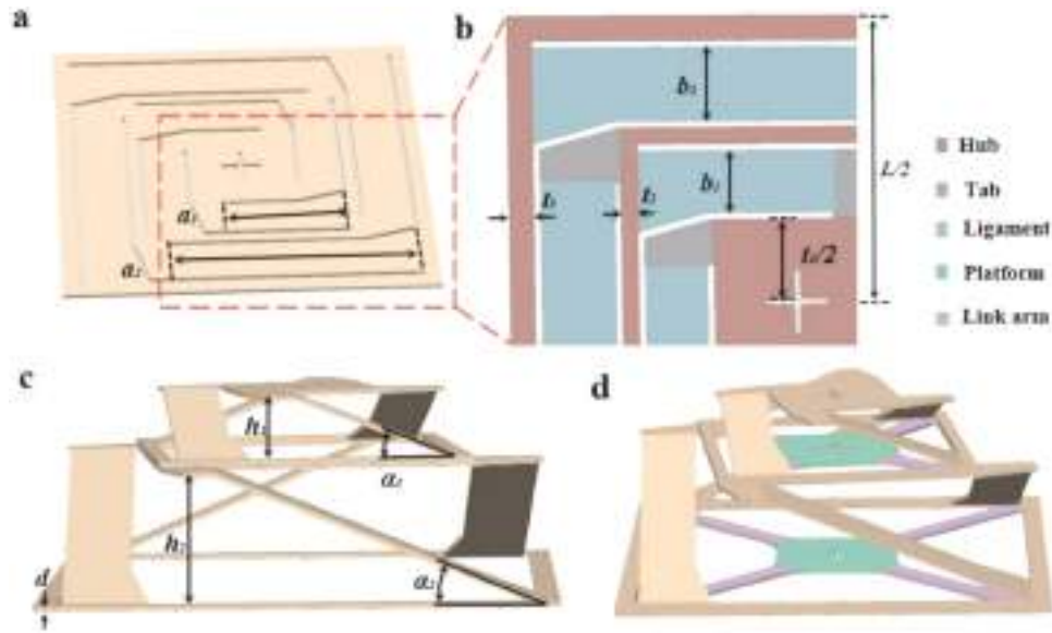
Fig. 1. Schematic diagram of the 2D plane and 3D state of the PKMM structure: (a) planar state. (b) component segmentation. (c) 3D state, and (d) assembled 3D state with integrated components.
