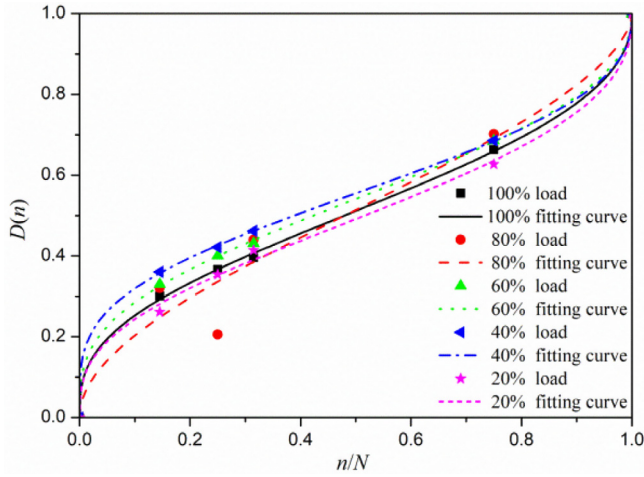
Fig. 7. The damage development curves under different loadings.
