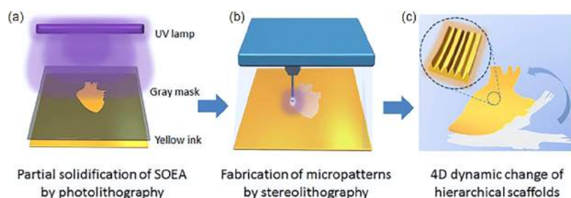
Figure 10 (Color online) Schematic of the photolithographic-sterolithographic-tandem process. (a) The exposed heart-shaped yellow ink was partially solidified under UV lamp; (b) micropatterns are drawn using a laser head on the unsolidified ink film forming hierarchical structures; (c) the 4D performance of the flat scaffold under external stimulus [49].
