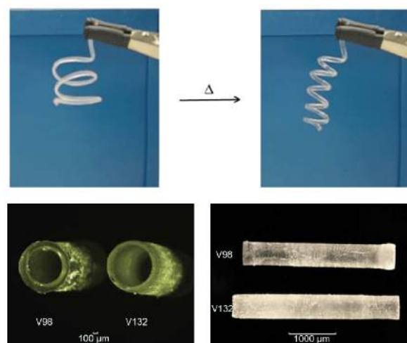
Figure 11 (Color online) Photographs of PTHF-DA shape memory microtubes printed via SLA. Shape changes can occur at room temperature and -20^\circ\text{C} [52].
