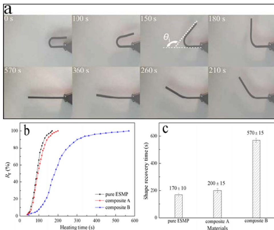
Figure 7. (a) Shape recovery process of composite B specimen, (b) typical relationship between shape recovery ratio ( R_r ) and heating time, and (c) shape recovery times of different materials at 120°. [Color figure can be viewed in the online issue, which is available at wileyonlinelibrary.com .]
