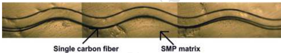
Figure 4.2. A typical post-buckling phenomenon: single carbon fiber in the shape memory polymer buckling, showing a similar sine wave form. [214]
