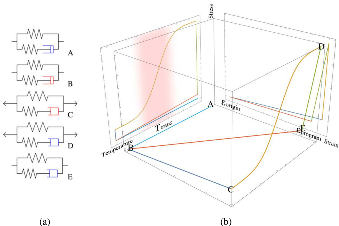
Figure 2.1. A typical hot programming, hot recovery, unloaded dual-shape memory cycle and the SLS model corresponding to the state of each stage. In this figure, the blue dashpot indicates that the viscosity of the dashpot is at its maximum (at room
