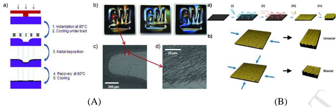
Figure 3.6. Surface structure of shape memory polymer created by buckling. (A) one-dimensional sinusoidal corrugated surfaces. (a) Schematic of production progress, (b) photo and (c) microstructure photo. (B) One-/two-dimensional sinusoidal corrugated surfaces. (a) Schematic of production progress. (b) Uniaxial and biaxial recovery create different shapes.[54][55]
