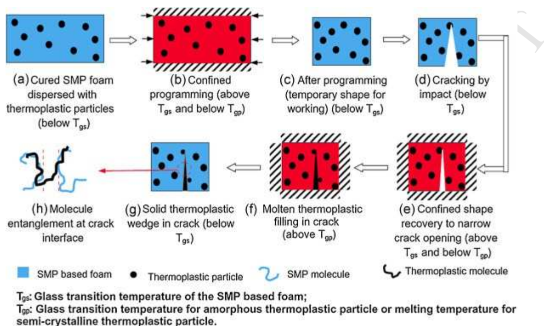
Figure 3.4. Schematic of self-healing progress of shape memory polymer-based smart foam, showing an example of close-then-heal (CTH). [50]
