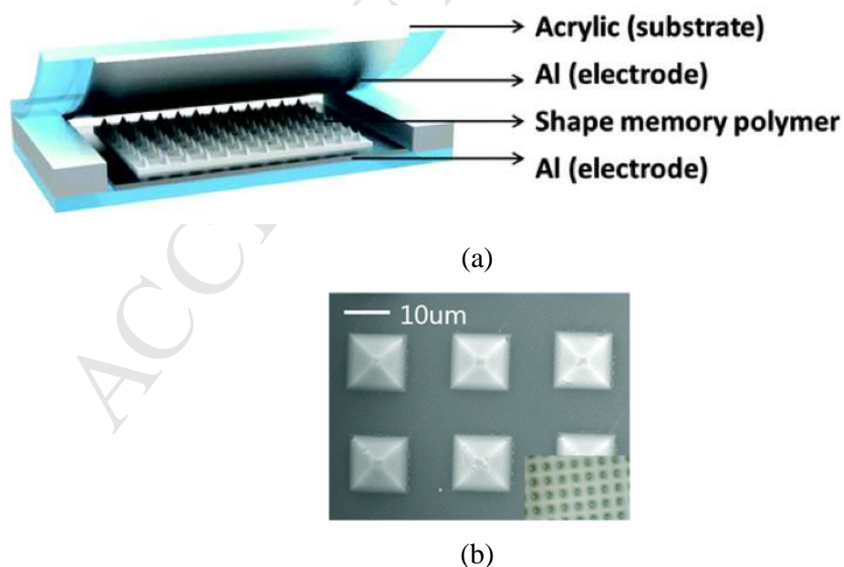
Figure 5.4. Shape memory polymer-based self-healing triboelectric nanogenerator. (a) Schematic of the PU-TENG structure. (b) PU pyramid pattern on the PU triboelectric layer.[24]
