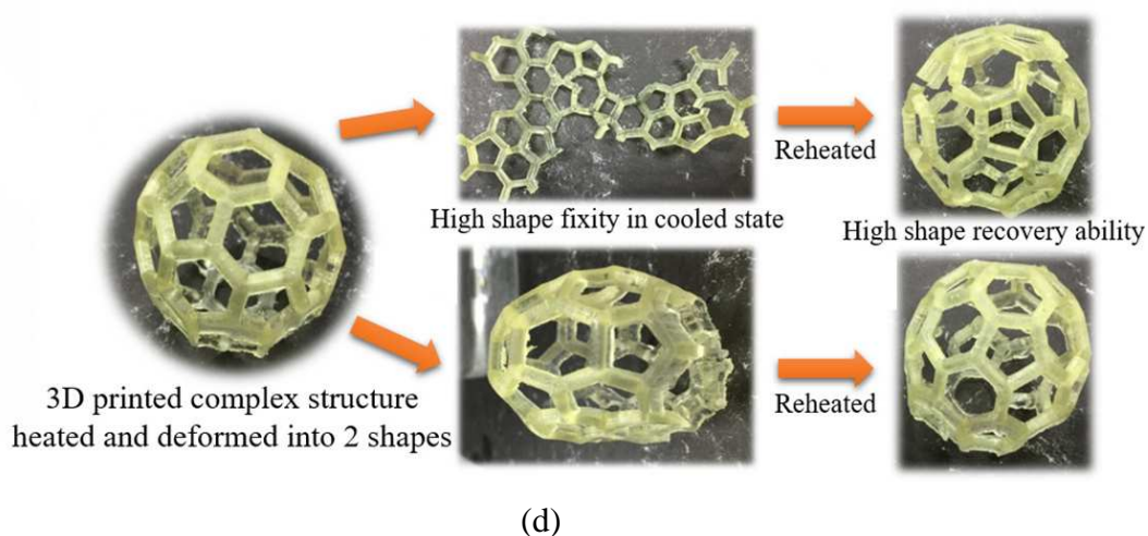
Figure 5.5. 3D printing product of shape memory polymers and composites. (a) 3D printing of the Eiffel Tower based on shape memory polymers, with meticulous detail and outstanding ability to recover. (b) SMPC 3D printing based on ESBO and
