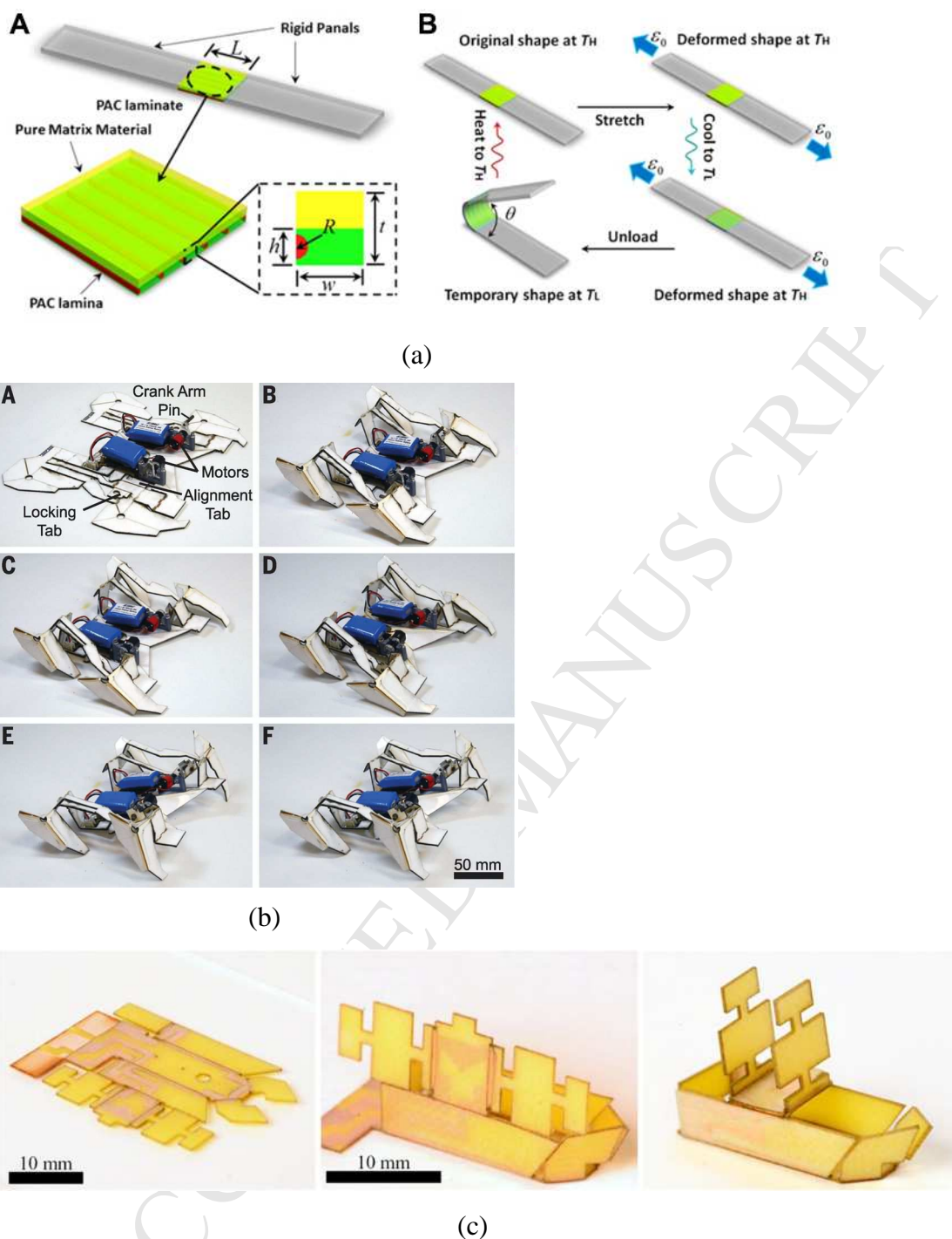
Figure 5.6. Origami is achieved by laminating an SMPC. (a) Schematics of a PAC hinge and programming progress. In essence, this folding is also a loaded shape memory cycle produced by stretching at high temperatures. After the external load is released, the hinge is bent to the designed angle because of the competition between the base material and the shape memory material. Afterward, the hinge can be reheated and reused. (b) Creation of a movable robot based on origami. The figure shows the robot at each stage of assembly, three of which are self-folding. (c) A boat
