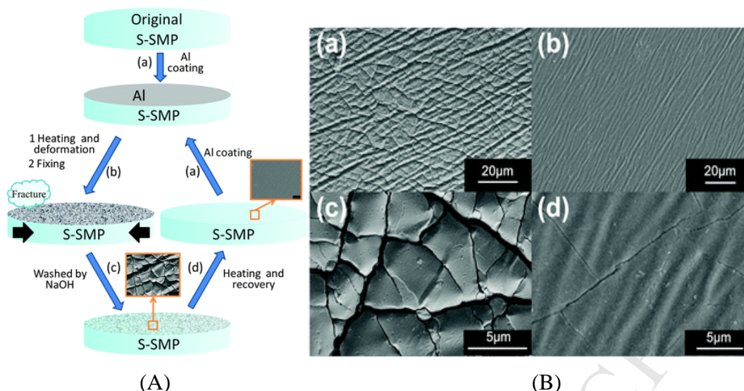
Figure 3.5. Controlled wettability based on reversible micro-cracking on a shape memory polymer surface. (A) Schematic of the process of hydrophobicity change. (B) Microstructure photos. (a,c) As the film cracks, the polymer substrate is exposed, so the surface shows a hydrophilic nature. (b,d) Metal cracks in contact with the surface of the material showing the hydrophobicity of the metal.180
