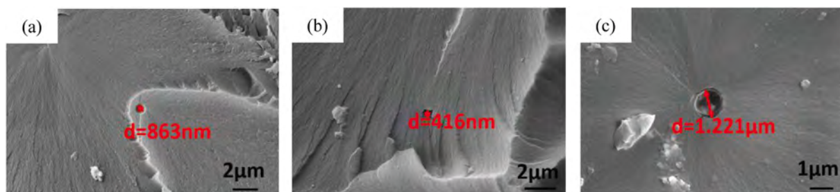
Fig. 20. SEM images of tensile fractured surfaces, a bubble in (a) X-0.02 sample, (b) X-0.05 sample and (c) direct casting sample [18].
